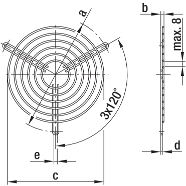
Guard grilles for centrifugal blowers with dual inlet (versions with EW motor)
