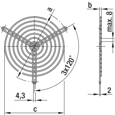
Guard grilles for centrifugal blowers with dual inlet
